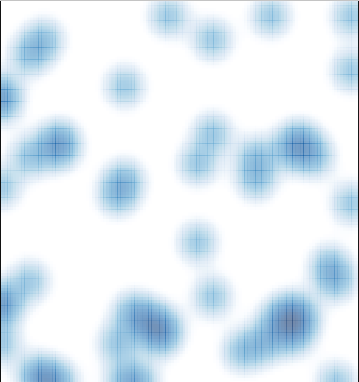
# features = 52 , max = 2
